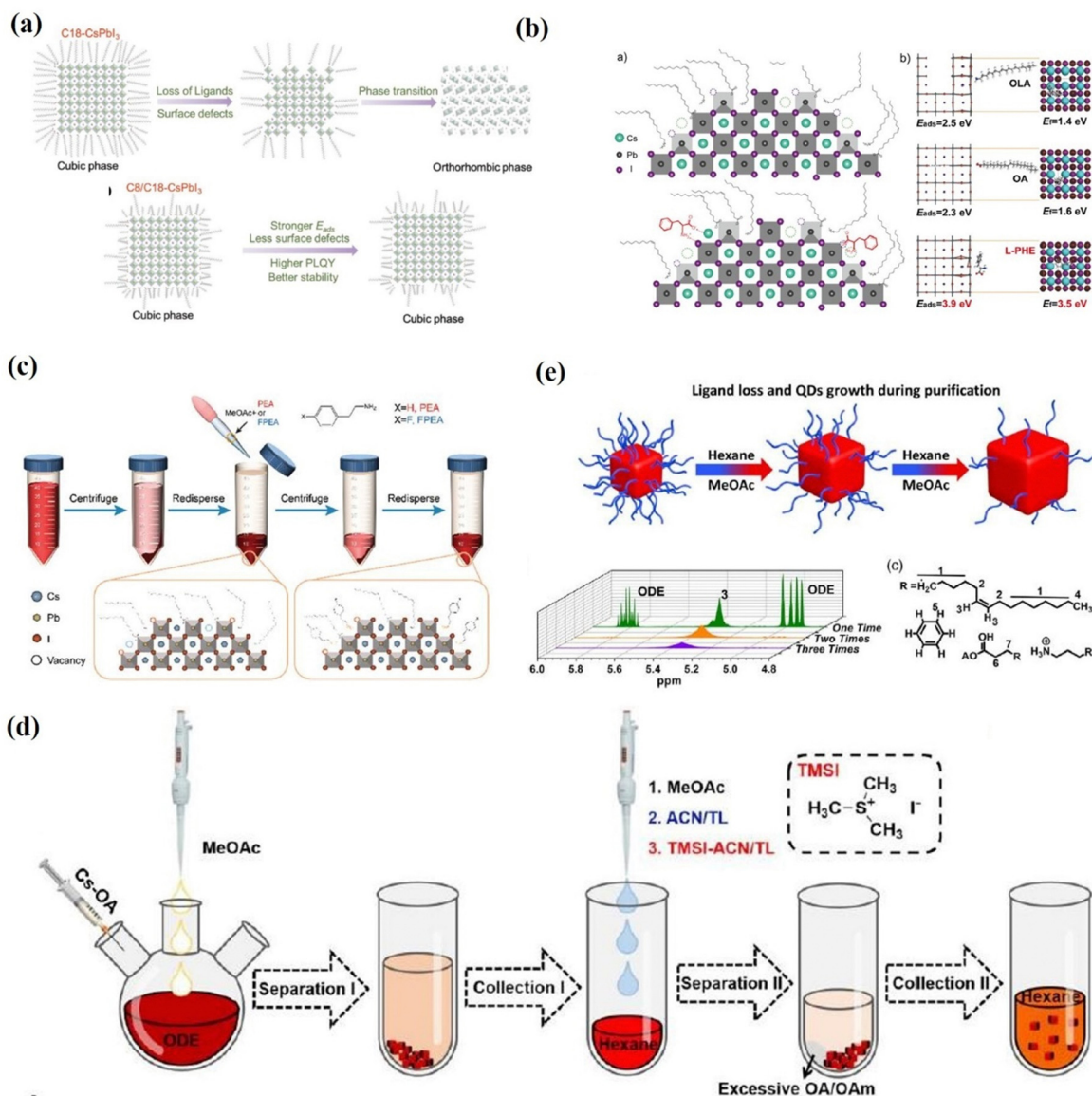
Fig. 17 (a) Schematic of the \text{CsPbI}_3 \alpha -phase stabilization mechanism due to the presence of C8. Reproduced with permission from ref. 169. Copyright 2019, Wiley-VCH. (b) Schematic of the surface of the as-synthesized \text{CsPbI}_3 perovskite QDs with and without L-PHE passivation and the DFT calculated adsorption energy ( E_{\text{ads}} ) of OA, OAm and L-PHE ligands on the optimized \text{CsPbI}_3 surfaces, and the corresponding formation energy of vacancy ( E_f ) on \text{CsPbI}_3 surfaces after the adsorption of different ligands. Reproduced with permission from ref. 170. Copyright 2020, Wiley-VCH. (c) A schematic diagram of the pseudo-solution-phase ligand exchange (p-SPLE) process. Reproduced with permission ref. 171. Copyright 2021, The Royal Society of Chemistry. (d) Schematic presentation of the purification processes of PQDs, in which the ligand riveting treatment was conducted after the "Collection I" process. Reproduced with permission ref. 172. Copyright 2022, The Royal Society of Chemistry. (e) A schematic illustration of QD changes during treatments and the full ^1\text{H} NMR spectrum of the 1–3 times treatments of \text{CsPbBr}_2 QDs in deuterated chloroform. Reproduced with permission from ref. 173. Copyright 2020, Wiley-VCH.
