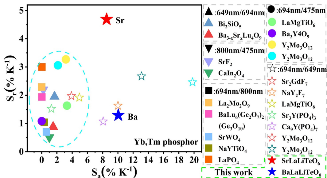
Fig. 8 Comparison of thermometry sensitivity between AlLaLiTeO_6:5\%Yb^{3+},0.2\%Tm^{3+} and other Yb^{3+} and Tm^{3+} co-doped phosphors.
