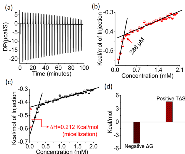
Fig. 2 (a) Measurement of heat release by ITC upon injection of a nanoaggregate solution of LPA into pure water at 298 K. (b) CAC determination from a plot of enthalpy vs. concentration. (c) Calculation of \Delta H of aggregation from a plot of \Delta H vs. concentration. (d) Plot showing negative \Delta G and positive \Delta S . Experimental temperature = 298 K.
