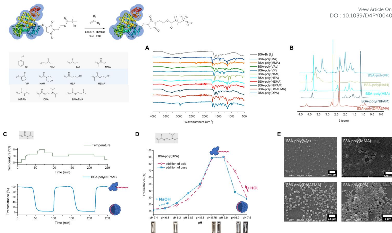
Figure 3. Characterization of amphiphilic, hydrophilic, and responsive protein-polymer conjugates. A. IR spectra of the bioconjugates. B. ^1\text{H-NMR} spectra acquired for hydrophilic BSA-polymer conjugates. C. Transmittance vs. time curve at different temperatures showing the rapid response of BSA-poly(NIPAM). D. Transmittance vs. pH curves of BSA-poly(DPA). Two cycles are shown for the same sample in which the response was induced by changing the pH with the addition of HCl (pH decrease) or NaOH (pH increase). E. SEM and FE-SEM micrographs of amphiphilic protein-polymer conjugate nanoparticles.
