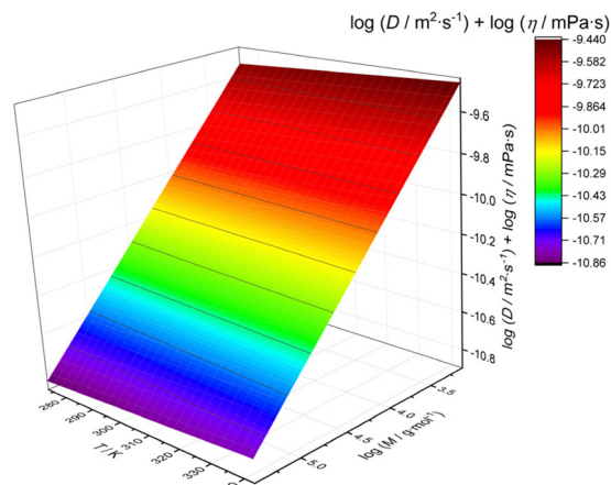
Fig. 3 3D calibration fit of viscosity-corrected diffusion coefficients (obtained using dstebpgp3s ) as a function of temperature and the molar mass of polystyrene standards.
