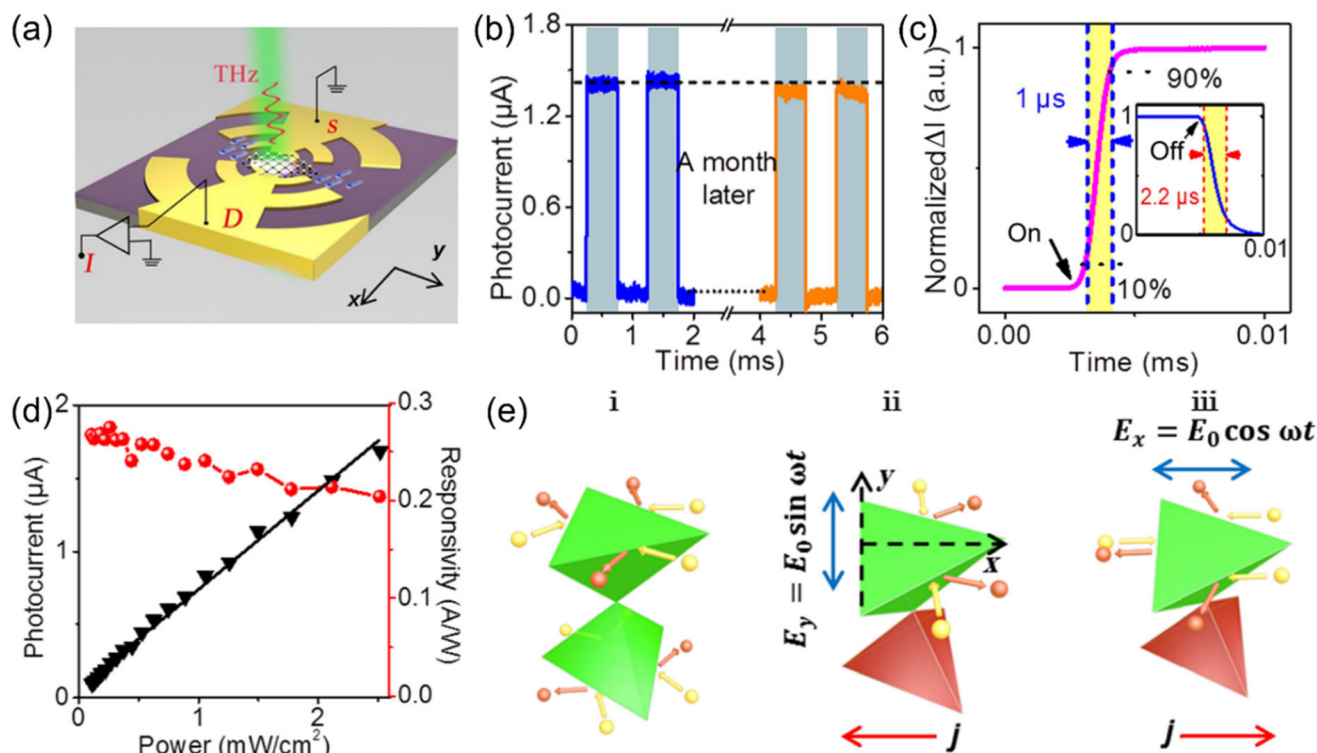
Fig. 17 (a) Schematic diagram of an MSM-type \text{PdTe}_2 terahertz detector. (b) Photoswitching curves under zero bias of a \text{PdTe}_2 device right after fabrication (blue line) and after storage in air for one month (orange line). (c) Temporal photoresponse. (d) Photocurrent (black line and triangles) and responsivity (red line and circles) as a function of light power density. (e) Schematic illustration of the working mechanism for the self-driven photoresponse. Reproduced from ref. 200 with permission from American Association for the Advancement of Science, copyright 2020.
