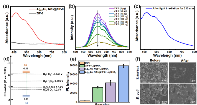
Fig. 4 (a) UV-visible DRS spectra of Ag 28 Au 1 NCs@ZIF-8 and ZIF-8. (b) PL emission spectra of Ag 28 Au 1 NC solution in the presence of different amounts of ZIF-8. (c) UV-visible DRS spectrum of Ag 28 Au 1 NCs@ZIF-8 after light irradiation for 210 min. (d) The diagram of energy levels of Ag 28 Au 1 NCs@ZIF-8. (e) The PL intensity of DCF treated with PBS under dark conditions (control group), and that with antibacterial agents under light irradiation and O 2 bubbling for 20 min. (f) SEM images of the bacteria before and after the photodynamic antibacterial test.
