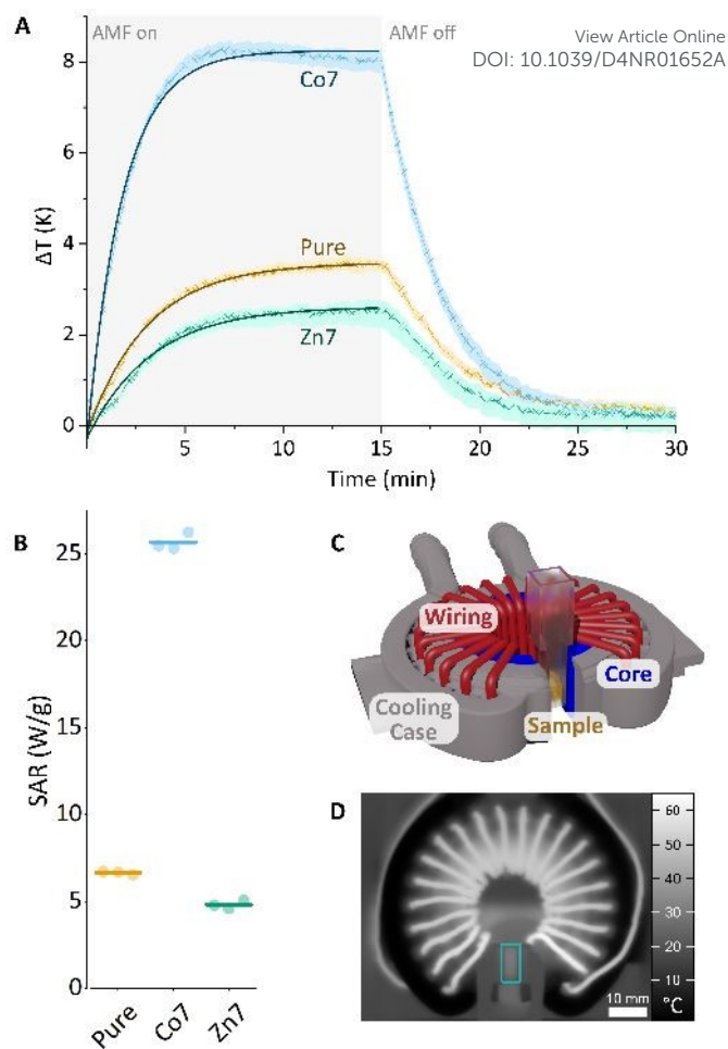
Figure 6 – (A) Hyperthermia measurement. Temperature kinetics of pure, Co7, and Zn7 MFT sample (each 35 \mu M) during exposure to the alternating magnetic field (45 mT, 93.75 kHz). Each curve is an average of three runs. The absolute temperature change \Delta T refers to the temperature increase above the temperature of pure buffer solution. All MFT and buffer solution samples measured in an identical manner. (B) Specific Absorption Rate (W/g) of each run (coloured dot) and average value (coloured line). (C) Custom-made hyperthermia setup. (D) Selected thermal image of that was taken during hyperthermia measurement, with the sample (blue box) in the centre of the magnet gap.
