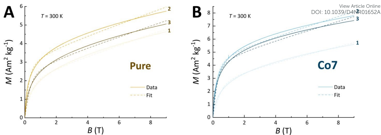
Figure S3 - Langevin Fits.
