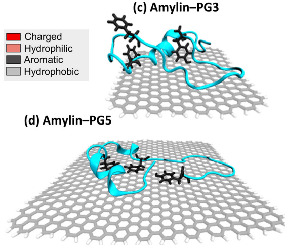
Fig. 2 Specific interactions between amylin and pristine graphene. (a) Average minimum distances measured between individual amylin residues and the PG3, PG5, and PG7 surfaces. Calculated on the lowest energy states of each system (shown in Fig. 1), with errorbars representing standard deviation. Shaded grey on the plot is used to indicate residue–NF contacts, defined as distances less than 0.4 nm. Residue numbers are coloured by sidechain physicochemical properties: dark red – charged (Lys and Arg); light red – hydrophilic (Asn, Thr, Gln, His, Ser and Cys); light grey – hydrophobic (Ala, Leu, Val, Gly and Ile); and dark grey – aromatic (Phe and Tyr). (b)–(d). Representative snapshots that highlight favourable amylin–PG interactions. The amylin backbone is shown in cyan cartoon representation, residue sidechains are drawn in licorice atomic detail and coloured based on their properties ( i.e. , charged, hydrophilic, hydrophobic, and aromatic), and graphene carbon atoms are shown in grey with either space-filling (b) or licorice (c and d) representations. Water and ions are hidden for clarity. (b) Top-view of amylin–PG5 showing residues within 0.4 nm of the NF. (c), (d). Side-view of amylin interacting with PG3 and PG5, emphasising the orientation of aromatic residues relative to the substrates.
