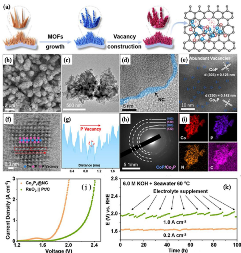
Fig. 8 (a) Schematic diagram illustrating the synthesis process for \text{Co}_x\text{P}_y@NC ; (b) SEM image and (c) TEM image of \text{Co}_x\text{P}_y@NC ; (d and e) HRTEM images and (f) STEM-BF image of \text{Co}_x\text{P}_y@NC ; (g) intensity profile obtained from the corresponding areas in part (f); (h) SAED pattern and (i) EDS mapping of \text{Co}_x\text{P}_y@NC for Co, P, N and C; (j) LSV curves for \text{Co}_x\text{P}_y@NC//\text{Co}_x\text{P}_y@NC in comparison with those of the \text{RuO}_2||\text{Pt/C} couple in 1 M KOH with seawater; (k) chronopotentiometry curve of \text{Co}_x\text{P}_y@NC//\text{Co}_x\text{P}_y@NC in 6 M KOH with seawater at 60 °C (reproduced with permission from ref. 15. Copyright 2023, Elsevier Ltd).
