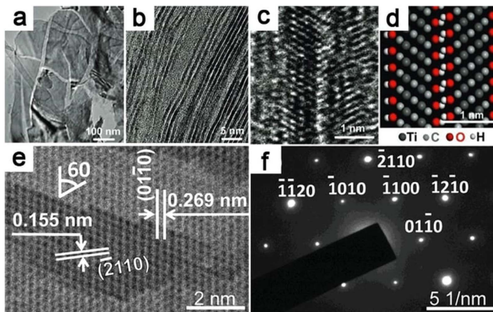
Fig. 10 SAED and TEM imaging of MXenes. (a) A TEM picture of exfoliated Ti–C–O–F 2D nanosheets. (b) MXene sheets with one or two layers. (c) HRTEM picture of bilayer Ti_3C_2(OH)_x F_y (d) its atomistic model of the layer structure (e) HRTEM image of multilayered MXene and (f) MXene's SAED pattern. 54
