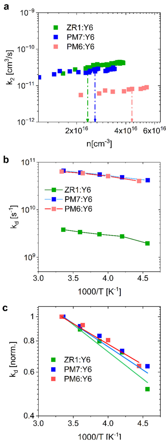
Fig. 4 (a) Bimolecular recombination coefficient versus charge carrier density of the ZR1:Y6, PM7:Y6 and PM6:Y6 devices measured with bias-assisted charge extraction with excitation energy of 2.07 eV at V_{OC} conditions. The data point for 1 sun illumination condition for each device is indicated with the dropping lines. (b) The dissociation rate coefficient ( k_d ) as a function of temperature for each system is shown. (c) Arrhenius fits (lines) to the normalized ( k_d ) as a function of temperature; entailing similar activation energies for charge generation.
