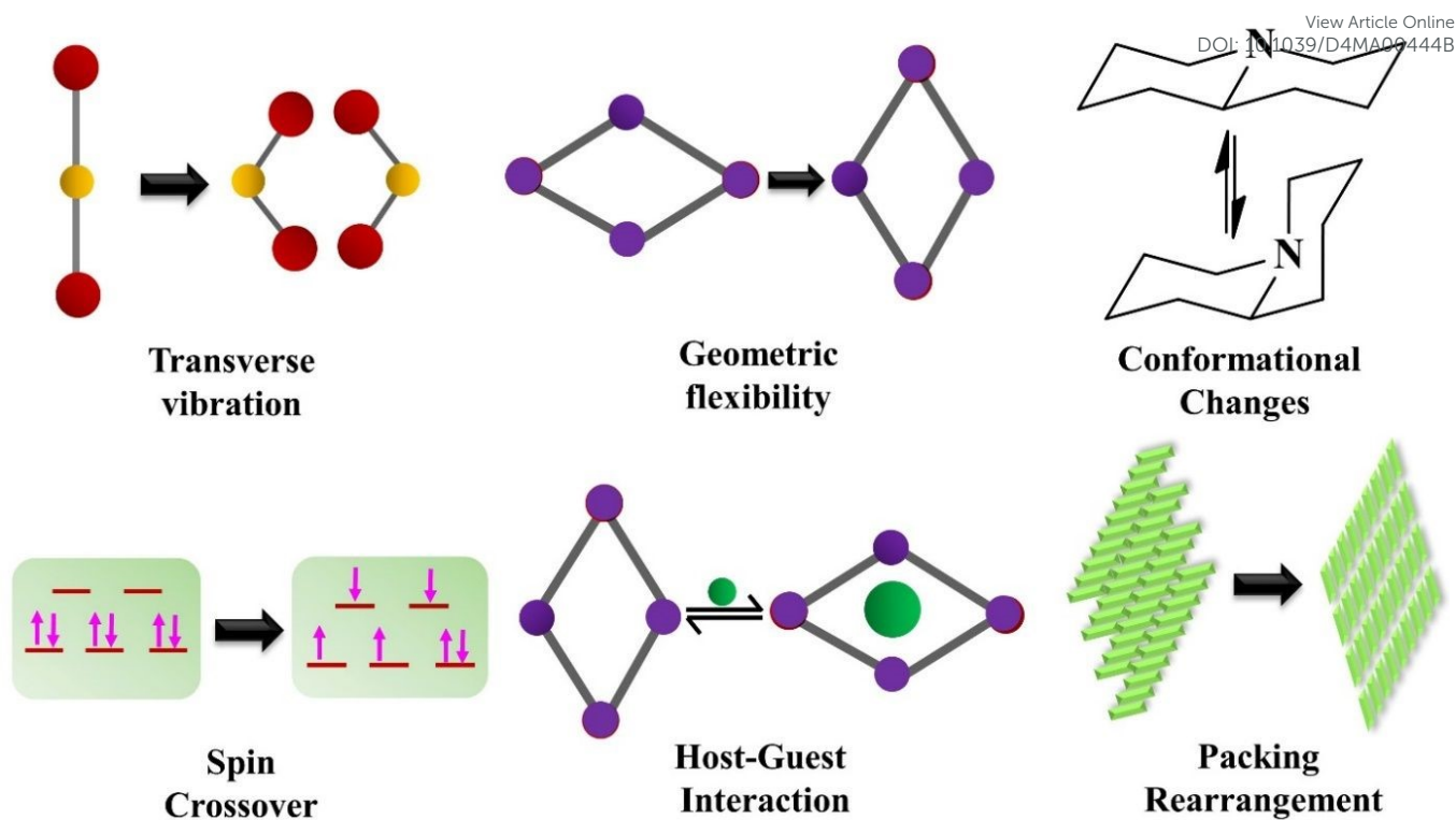
Figure 15: Various mechanisms leading to negative thermal expansion behaviour in molecular materials.
