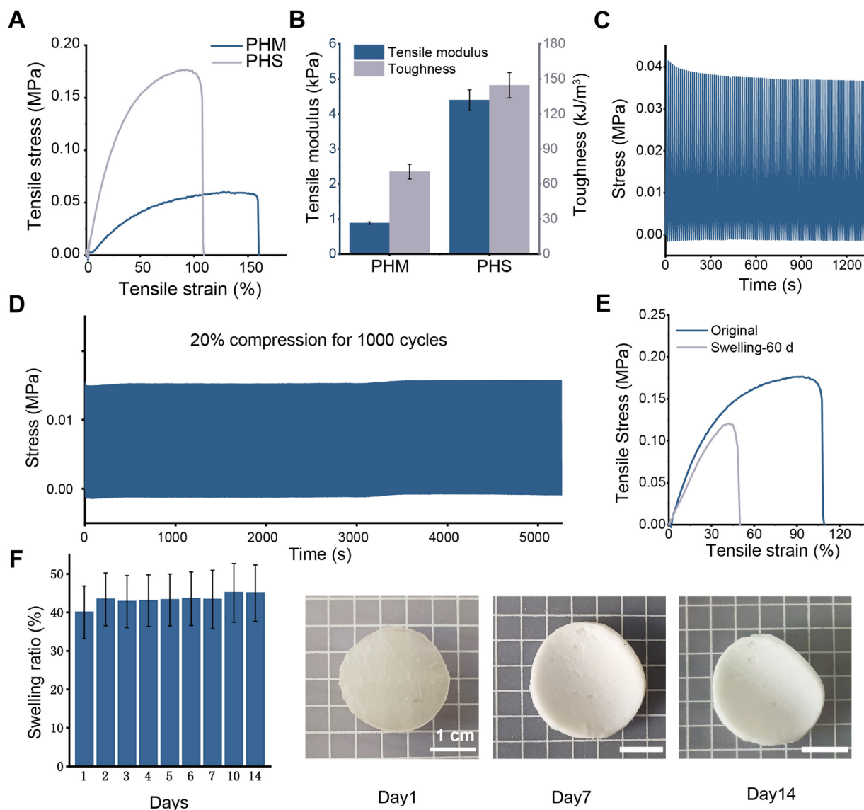
Fig. 2 Mechanical properties and swelling properties of the hydrogels. (A) and (B) Tensile stress-strain curves of PHM hydrogel and their corresponding tensile modulus and toughness histograms. (C) PHS hydrogel is subjected to 100 consecutive compression loading unloading curves at the maximum strain of 50%. (D) PHS hydrogel is subjected to 1000 consecutive loading unloading compression curves at the maximum strain of 20%. (E) Tensile stress-strain curve of PHM hydrogel before swelling and 14 days after swelling. (F) The swelling ratio of PHS hydrogel after 14 days and the physical pictures after 1, 7 and 14 days of swelling.
