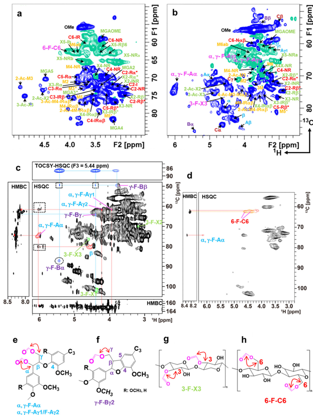
Fig. 7 Aliphatic sidechain region of 2D ^1\text{H} - ^{13}\text{C} HSQC spectra and 2D ^1\text{H} - ^{13}\text{C} HMBC and 3D TOCSY-HSQC NMR of the fractions from the Eucalyptus film formed at 50 ^\circ\text{C} . (a) Aliphatic sidechain region of 2D ^1\text{H} - ^{13}\text{C} HSQC spectrum from the aqueous fraction characterized as the polysaccharide-rich fraction. The signals belonging to cellulose, glucuronoxylan, glucomannan, and formylated compounds were presented in red, green, yellow/red, and pink, respectively. (b) Aliphatic sidechain region of the 2D ^1\text{H} - ^{13}\text{C} HSQC spectrum from the 2MeTHF fraction characterized as the lignin-rich fraction. The lignin linkages of \beta -O-4, \beta - \beta , \beta -5, and lignin-carbohydrate complex (LCC) are shown in blue, brown, purple, and yellow, respectively. Free \beta -O-4 lignin units are distinguished as \text{A}\alpha and \text{A}\beta to those of LCC as \alpha and \beta . The mannose unit of glucomannan was presented as 1 M to M6/M6' in yellow. The signal assignment is summarized in Tables S6 and S7 (ESI ^\dagger ). (c) NMR spectra of the aliphatic region of the lignin-rich-2MeTHF fraction. Signals from the formylated \alpha and \gamma positions of the \beta -O-4 unit are labelled as \alpha, \gamma\text{-F-A}\alpha and \alpha, \gamma\text{-F-A}\gamma 1/\text{F-A}\gamma 2 , respectively. Those from the \gamma position in \beta -5 and 3 positions of xylose units in xylan are labelled as \gamma\text{-F-B}\alpha/\gamma\text{-F-B}\beta and 3-F-X3, respectively. Signals in the dot squares and circles in the HSQC box are the inter-unit correlations of formylated \beta -O-4 and \beta -5, respectively. The 3D TOCSY-HSQC spectrum is the F1-F2 plane sliced at F3 = 5.44 ppm (the proton resonance of \beta -5 \alpha ). Signals of \beta -O-4, \beta -5, and xylose units are shown in blue, purple, and green, respectively. (d) Aliphatic region of 2D ^1\text{H} - ^{13}\text{C} HSQC and HMBC spectra of the precipitate. The signal of formylated 6-OH of glucose residues in cellulose is labelled 6-F-C6. The \alpha position of the \beta -O-4 unit in lignin is labelled as \alpha, \gamma\text{-F-A}\alpha . Correlation of formyl units with \alpha and \gamma positions in \beta -O-4 (e), \gamma position in \beta -5 (f), the 3rd position of the xylose residue in xylan (g), the 6th position of the glucose residue in cellulose (h).
