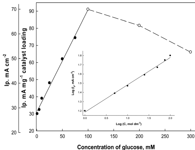
Fig. 10 Effect of glucose concentrations on the oxidation peak current densities of glucose in 0.5 M NaOH at 0.02 \text{ V s}^{-1} (from cyclic voltammograms, not presented), and the inset plot represents the logarithmic relationship between the concentrations and the oxidation peak current densities.
