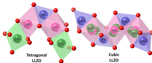
Fig. 2 The Li-positions in tetragonal and cubic LLZO. In tetragonal LLZO, the Li-ions occupy the 8a-tetragonal (Li1), 16f-octahedral (Li2) and 32g-octahedral (Li3) sites. In cubic LLZO, there are two sites, 24d-tetragonal (Li1) and 96h-octahedral (Li2). Li2 can also occupy the 48g position in the same octahedral void interchangeably.
