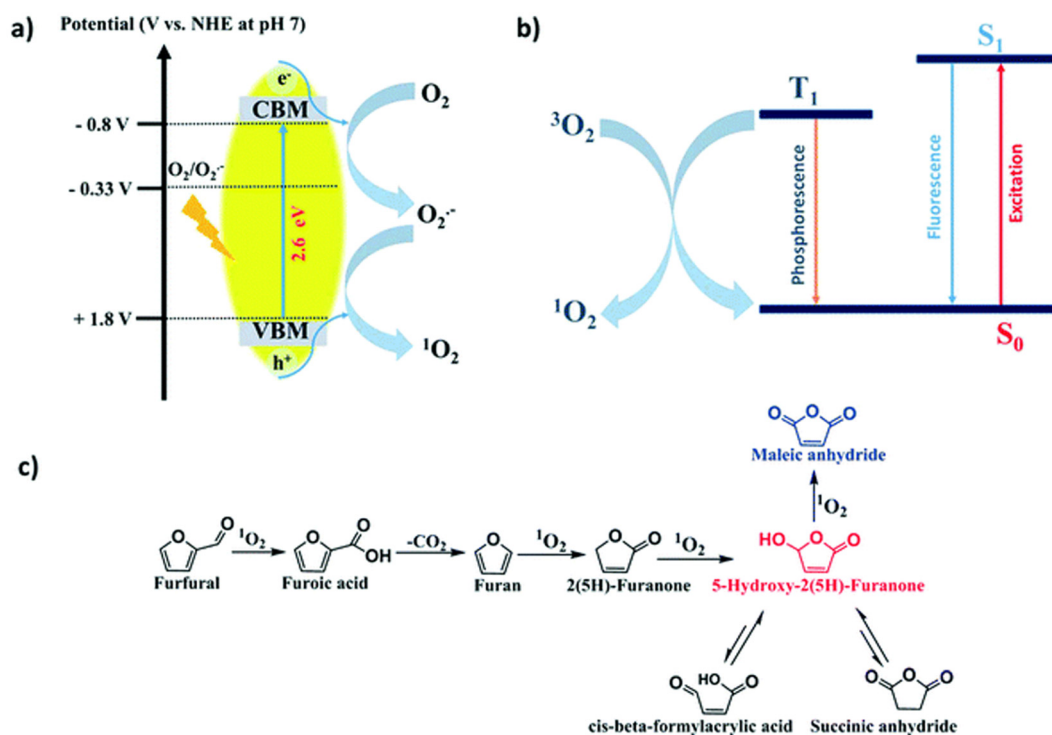
Fig. 22 (a) Generation of ^1\text{O}_2 on the surface of SGCN via h\nu , (b) ^1\text{O}_2 generation via triplet state energy transfer, and (c) plausible mechanistic pathway of FAL photooxidation. Reproduced from ref. 36, with permission of Royal Society of Chemistry, Copyright 2022.
