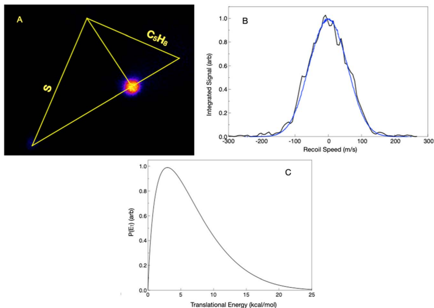
Fig. 6 (A) Velocity map image of the 99 u product, \text{C}_5\text{H}_7\text{S} , for the reaction of S(^3P) with isoprene (Newton diagram superimposed) under a collision energy of 14.0 \text{ kcal mol}^{-1} . (B) Total signal from the image in (A) projected onto the x -axis and transformed into a speed distribution (black). The simulated image using the velocity distribution is then projected to produce a profile (blue) that closely matches the observed one. (C) Total translational energy release ( P(E_T) ) extracted following analysis of the image in (A).
