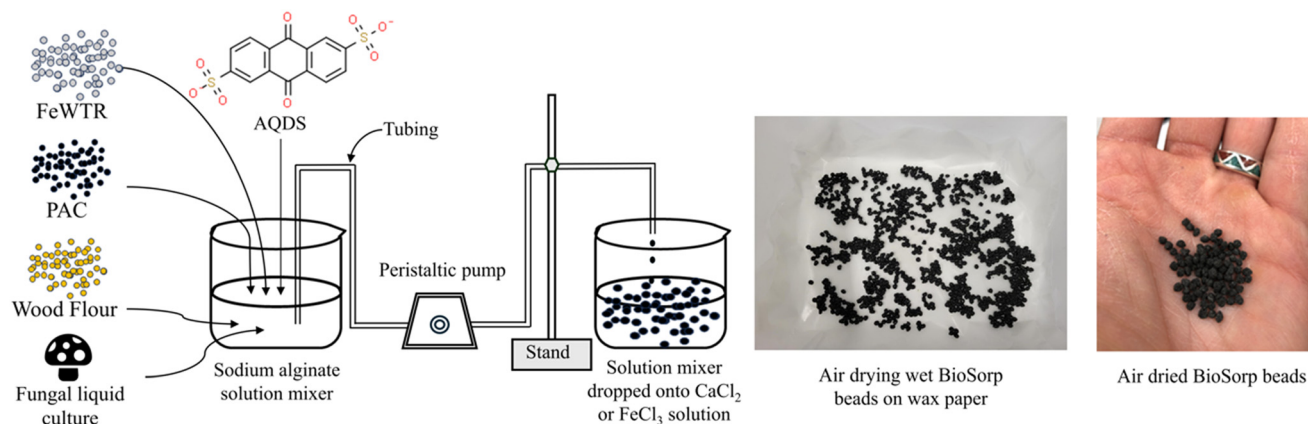
Fig. 1 Schematic diagram of BioSorp bead making procedure. The final beads containing the encapsulated materials and culture are approximately 3 mm in diameter and hard to the touch (FeWTR = iron water treatment residual; PAC = powdered activated carbon, AQDS = anthraquinone-2,6-disulfonate).
