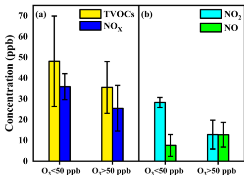
Fig. 4 (a) The concentration of TVOCs in the high O_3 region and the low O_3 region; (b) the concentration of NO_x in the high O_3 region and the low O_3 region.
