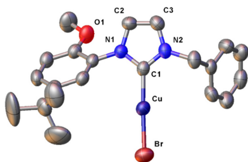
Fig. 5 ORTEP drawing of complex [\text{CuBr}(\mathbf{a}^1)] . Ellipsoids are drawn at the 50% probability level. Hydrogen atoms have been omitted for clarity. Selected bond distances (Å) and angles ( ^\circ ): Cu–C1 1.890(6) , Cu–Br 2.2273(9) , C1–Cu–Br 178.3(2) .
