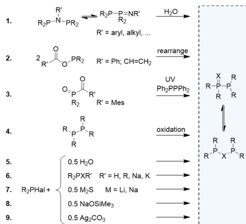
Fig. 3 Various synthetic strategies for the formation of PPX/PXP-type ligands. \text{R} = (\text{fluorinated}) \text{ alkyl}, \text{aryl}, \text{OR} , or \text{NR}_2 .
