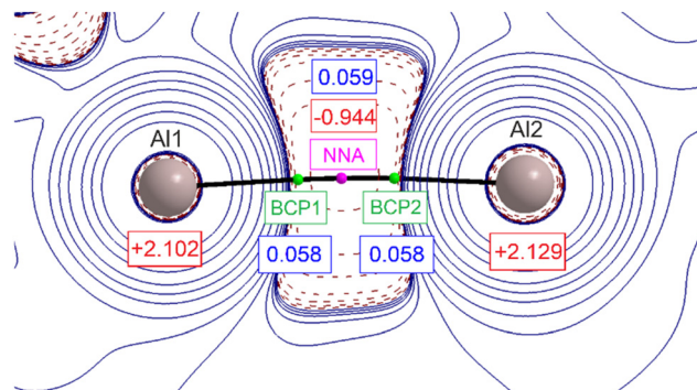
Fig. 3 Laplacian operator of the electron density in a plane containing both Al nuclei of [(DNI(H)Al) 2 ] ( 2 ). Contours are drawn in a logarithmic scale: positive as solid blue lines and negative ones as dashed red lines. The non-nuclear attractor (NNA) is depicted in a magenta box, bond critical points (BPCs) are given in green box, and AIM charges are given in red boxes for both Al ions and charge density magnitude at both bond critical points and the NNA are given in blue boxes ( \text{e}^- \text{ Bohr}^{-3} ).
