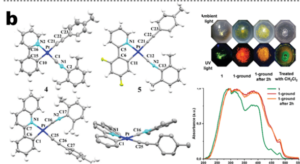
Fig. 19 (a) Schematic illustration of excitation-wavelength-dependent emission of a Pt(II) complex 5-8 and their spectra observations. Reproduced from ref. 123 with permission. Copyright (2021), American Chemical Society. (b) Crystal structures of complex 5-9 to 5-11 and their MCL observations. Reproduced from ref. 122 with permission. Copyright (2020), The Royal Society of Chemistry.
