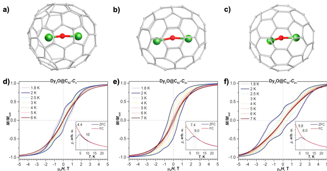
Fig. 6 Molecular structures of \text{Dy}_2\text{O}@\text{C}_{82} (a), \text{Dy}_2\text{O}@\text{C}_{3v}(8) (b) and \text{Dy}_2\text{O}@\text{C}_{2v}(9) (c). Magnetic hysteresis curves of \text{Dy}_2\text{O}@\text{C}_{82} (d), \text{Dy}_2\text{O}@\text{C}_{3v}(8) (e) and \text{Dy}_2\text{O}@\text{C}_{2v}(9) (f) in the range of 1.8–7 K using a field sweep rate of 2.9 \text{ mT s}^{-1} . The insets represent their corresponding ZFC/FC curves at an applied magnetic field of 0.2 T with a temperature sweep rate of 5 \text{ K min}^{-1} . Reproduced from ref. 102.
