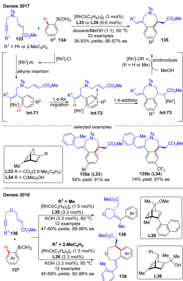
Scheme 39 Rh(I)-Catalyzed arylative cyclization of N - or O -tethered alkyne enoates with arylboronic acids.
