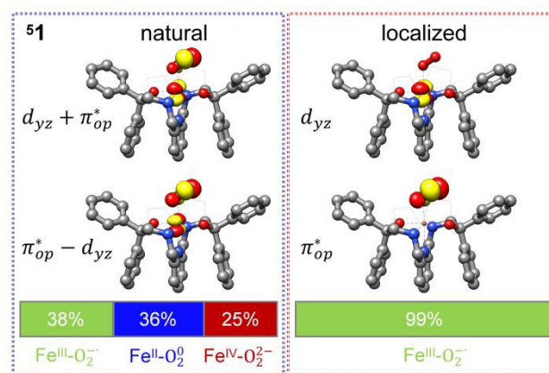
Fig. 3 d_{yz} and \pi_{op}^* MOs in natural and localized forms with the electron configurations and their weights for ^5\mathbf{1} complex; Fe^{III}-O_2^- denotes the electron configuration of d_{xz}^1 (d_{yz} + \pi_{op}^*)^1 d_{xy}^1 d_{x^2-y^2}^1 (d_{z^2} - \pi_{ip}^*)^1 \pi_{ip}^2 \pi_{op}^2 (\pi_{ip}^* + d_{z^2})^2 (\pi_{op}^* - d_{yz})^1 , Fe^{IV}-O_2^- represents the electron configuration of d_{xz}^1 (d_{yz} + \pi_{op}^*)^0 d_{xy}^1 d_{x^2-y^2}^1 (d_{z^2} - \pi_{ip}^*)^1 \pi_{ip}^2 \pi_{op}^2 (\pi_{ip}^* + d_{z^2})^2 (\pi_{op}^* - d_{yz})^2 , and Fe^{II}-O_2 indicates the electron configuration of d_{xz}^1 (d_{yz} + \pi_{op}^*)^2 d_{xy}^1 d_{x^2-y^2}^1 (d_{z^2} - \pi_{ip}^*)^1 \pi_{ip}^2 \pi_{op}^2 (\pi_{ip}^* + d_{z^2})^2 (\pi_{op}^* - d_{yz})^0 , ligand atoms are omitted for clarity.
