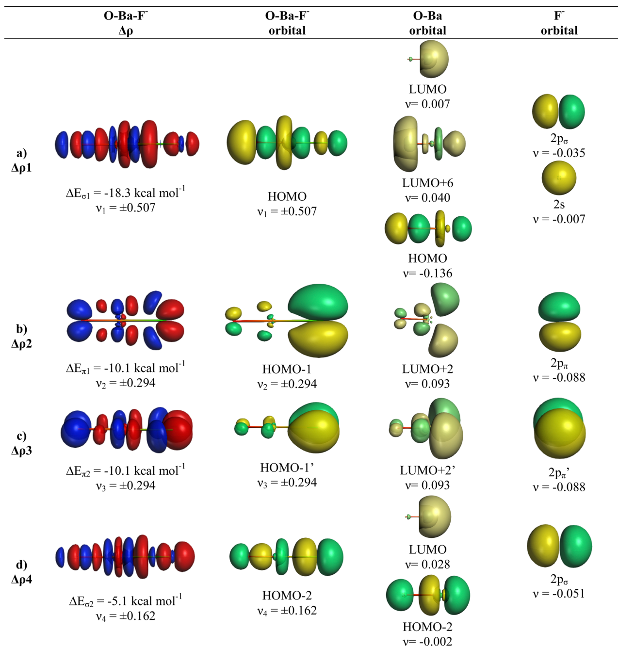
Fig. 10 Plot of deformation densities \Delta\rho of \text{OBaF}^- . The pairwise orbital interactions and the associated interaction energies ( \Delta E_{\text{orb}} ) between fragments OBa (S) and F^- (S) in \text{OBaF}^- of the linear structure, as well as the shape of the most important interacting MOs. The direction of the charge flow is red \rightarrow blue. (Isovalue 0.03e \text{ a.u.}^{-3} ).
