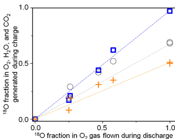
Fig. 11 Fractions of ^{18}\text{O} in \text{O}_2 (■), \text{H}_2\text{O} (+), and \text{CO}_2 (○) generated during charge as a function of the fraction of ^{18}\text{O} in the \text{O}_2 gas flow during discharge.
