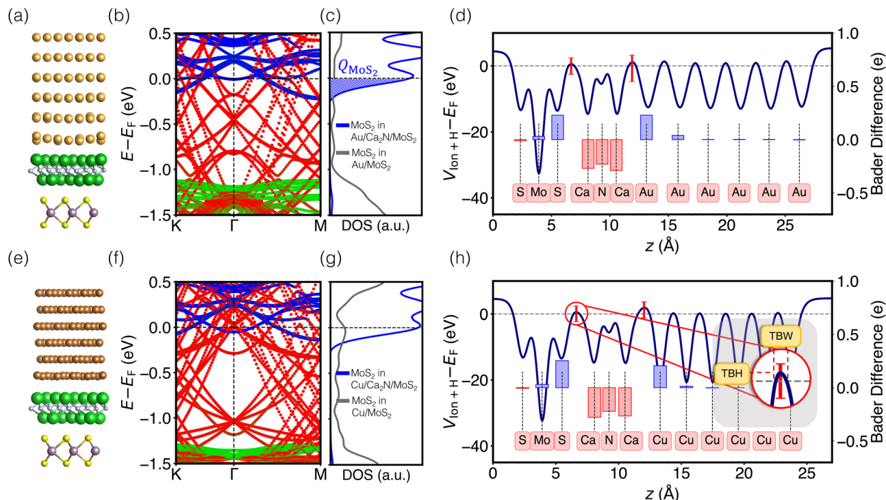
Fig. 2 (a) Optimized structure, (b) material-projected band structure, (c) densities of \text{MoS}_2 states per \text{MoS}_2 formula unit, and (d) electrostatic potential for the \text{Au}/\text{Ca}_2\text{N}/\text{MoS}_2 interface. Panels (e)–(h) present the same quantities for the \text{Cu}/\text{Ca}_2\text{N}/\text{MoS}_2 interface. Metal bands are coloured red, \text{Ca}_2\text{N} bands are coloured green, and \text{MoS}_2 bands are coloured blue. The shaded region of the DOS plot corresponds to Q_{\text{MoS}_2} . In the potential plots, the red bars indicate the range of values at the maximum point within the interface regions. The results are overlaid with the differences in Bader atomic charges for the heterostructures, relative to the separated materials. Positive (negative) values indicate accumulation (depletion) of electron density.
