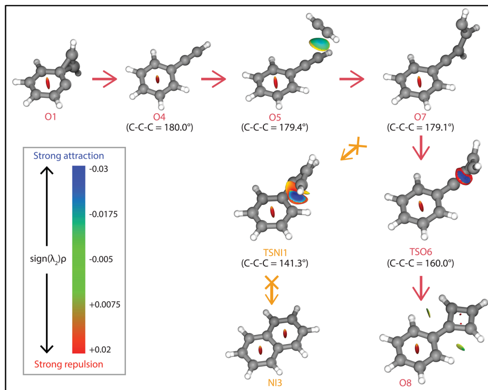
Fig. 8 NCI plots of intermediates and transition states of the reaction pathways towards phenylcyclobutadiene*+ ( O8 , red arrows), and naphthalene*+ ( NI3 , orange arrows). The strengths of the NCIs are shown by the color spectrum ranging from red (strong repulsion), green (weak attraction) and blue (strong attraction). The calculated angle of the C–C–C group is shown next to the structures.
