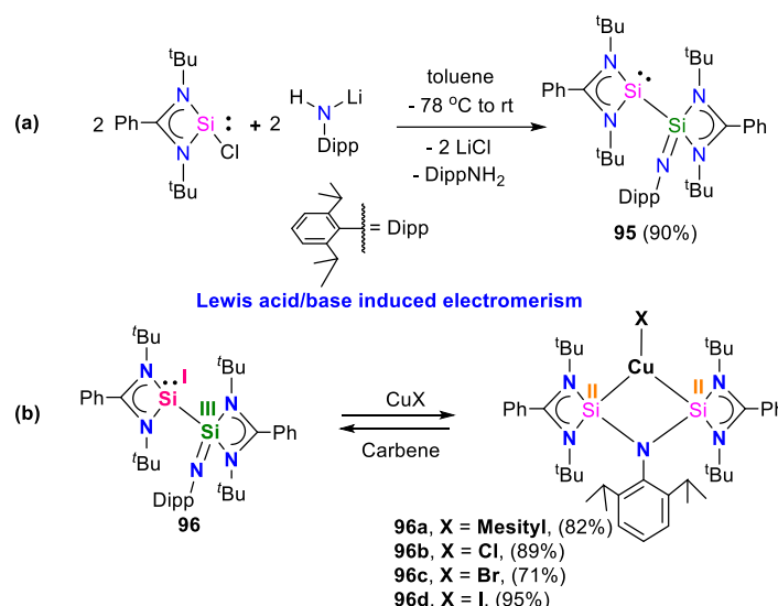
Scheme 36 Synthesis of 95 and its copper(I) complexes.
