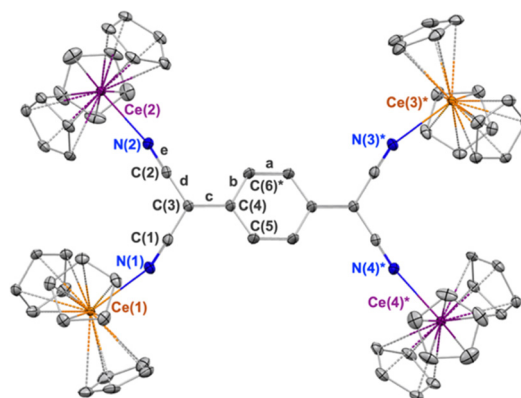
Fig. 1 Thermal ellipsoid plot of 1 shown at the 30% probability level. \text{Ce}^{\text{III}} centers are shown in orange and \text{Ce}^{\text{IV}} in purple color. The * indicates at equivalent position (-x, 1-y, 1-z) . Hydrogen atoms and co-crystallized toluene molecules are omitted for clarity.
