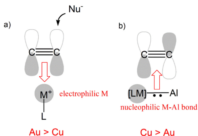
Scheme 9 (a) Electrophilic behaviour of [ML] + (M = Cu, Au) complexes for alkyne activation (Au more efficient than Cu); (b) nucleophilic behaviour of the M–Al (M = Cu, Au) bond in coinage metal–aluminyl complexes towards alkynes (Cu more efficient than Au).
