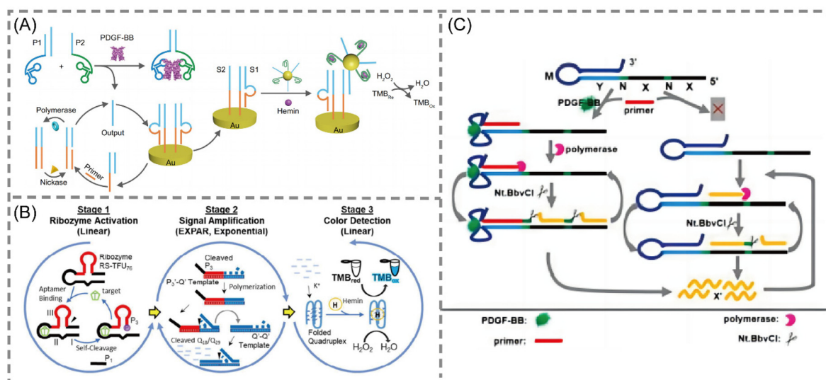
Fig. 5 Schematic representation of aptamer-based approaches. (A) A novel electrochemical biosensing platform on the basis of target-triggered proximity hybridization-mediated EXPAR for ultrasensitive protein analysis. 69 (B) A simple colorimetric system for detecting target antigens by a 3-stage signal transformation-amplification strategy. 70,71 (C) A rationally designed aptamer-based hairpin structure-switching EXPAR template for realizing protein triggering EXPAR (PTEXPAR). 74
