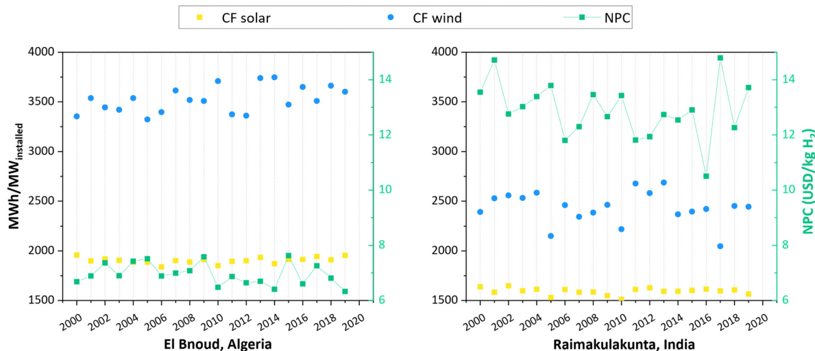
Fig. 3 Net production cost vs. annual availability of renewable energy. For this 20 years analysis, the annual NPC of green H 2 ranges from 6.3 to 7.6 USD per kg H 2 ,g (21% variation) in El Bnoud (Algeria) and from 10.5 to 14.8 USD per kg H 2 ,g (41% variation) in Raimakulakunta (India), respectively.
