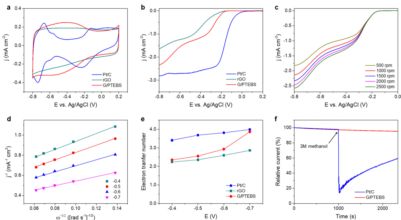
Fig. 5 (a) CV curves and (b) LSV curves (at 1500 rpm) of G/PTEBS, rGO and the commercial Pt/C electrocatalysts measured in 0.1 M KOH (scan rate: 50 \text{ mV s}^{-1} ). (c) RDE voltammograms (LSV curves) of G/PTEBS at increasing rotation speeds (scan rate: 10 \text{ mV s}^{-1} ). (d) K-L plots of the G/PTEBS electrocatalysts at different potentials. (e) Electron transfer numbers of G/PTEBS compared to those of rGO and the commercial Pt/C. (f) Chronoamperometric responses of G/PTEBS and the Pt/C catalyst with the addition of methanol at 1000 s.
