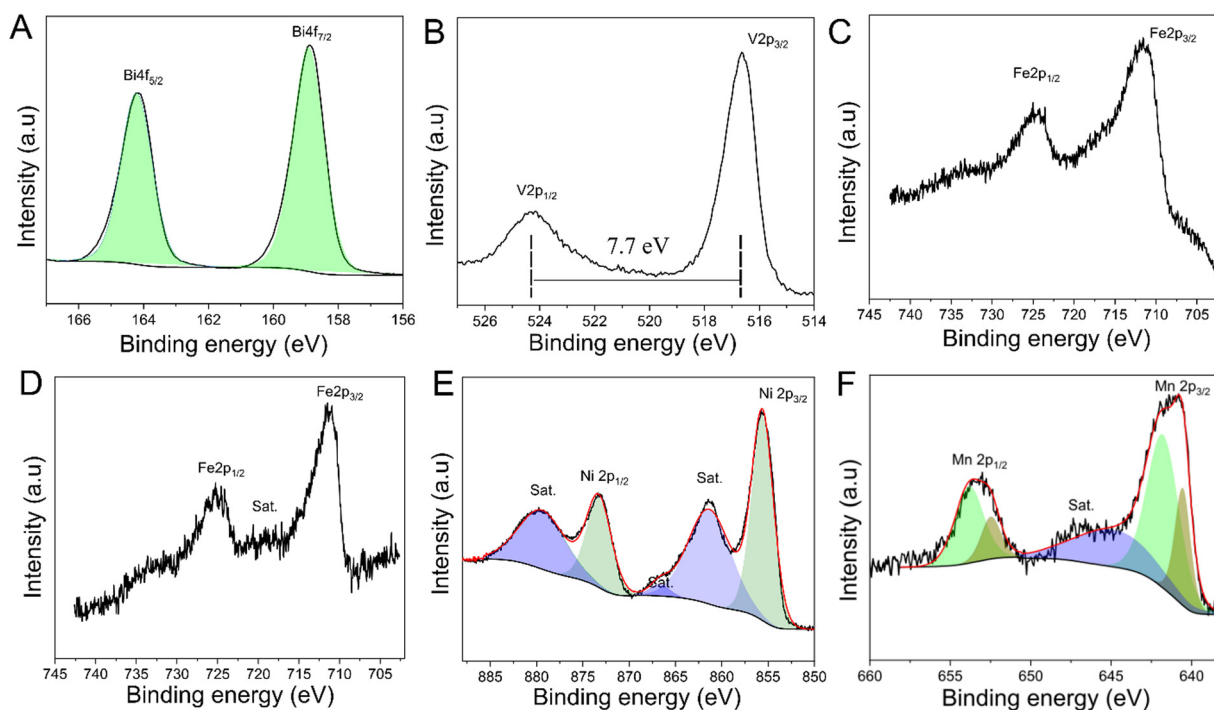
Fig. 2 XPS spectra of bare \text{BiVO}_4 at 400 °C for 1 hour: (A) Bi 4f and (B) V 2p. XPS spectra of as-sputtered \text{FeMO}_x ( M = \text{Ni, Mn} ) on BVO films: (C) Fe 2p with \text{FeNiO}_x deposited for 60 s, (D) Fe 2p with \text{FeMnO}_x deposited for 60 s, (E) Ni 2p with \text{FeNiO}_x deposited for 60 s, and (F) Mn 2p with \text{FeMnO}_x deposited for 60 s.
