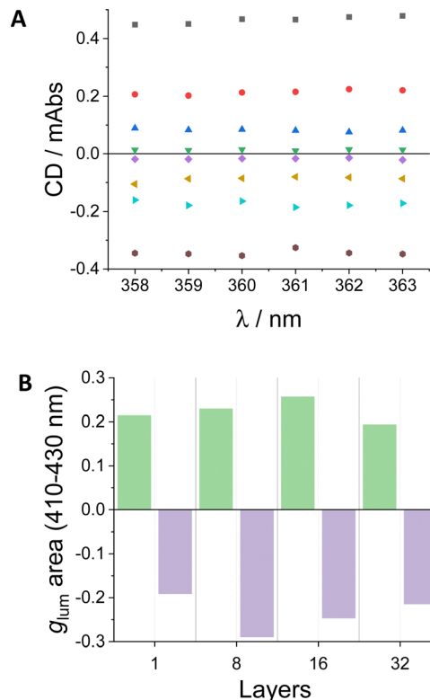
Fig. 9 (A) CD values of 1 (green inverted triangles), 16 (red circles) and 32 (black squares) layers of (S,S,P)-1, and 1 (purple diamonds), 8 (yellow triangles), 16 (light blue triangles) and 32 (gray circles) layers of (R,R,M)-1. (B) Integral of g_{lum} graph of (S,S,P)-1 (green areas) and (R,R,M)-1 (purple areas) layers in the selected wavelength region (410–430 nm). See Fig. S25 and S26 (ESI†) for raw data.
