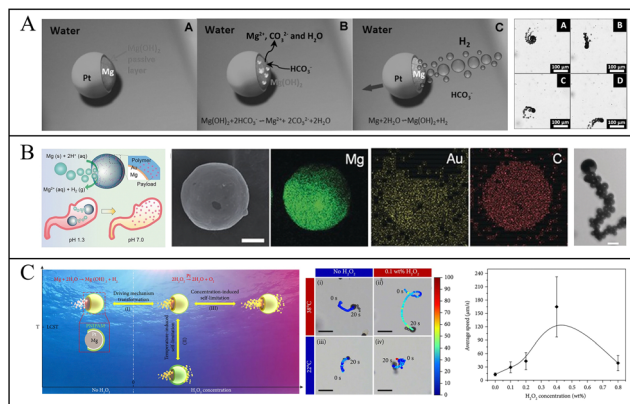
Fig. 3 Motion of Mg-based micromotors. (A) Etched \text{Mg(OH)}_2 on the surface of Mg-based Janus micromotors by \text{HCO}_3^- . Reproduced with permission. Copyright 2013, Wiley-VCH Verlag GmbH & Co. KGaA, Weinheim. 27 (B) Acid-responsive Mg-based micromotors moving in simulated gastric fluid. Reproduced with permission. Copyright 2017, Wiley-VCH Verlag GmbH & Co. KGaA, Weinheim. 67 (C) Mg-based Janus micromotors moving in response to variations in temperature and \text{H}_2\text{O}_2 concentration. Reproduced with permission. Copyright 2020, Kang Xiong et al. 70
