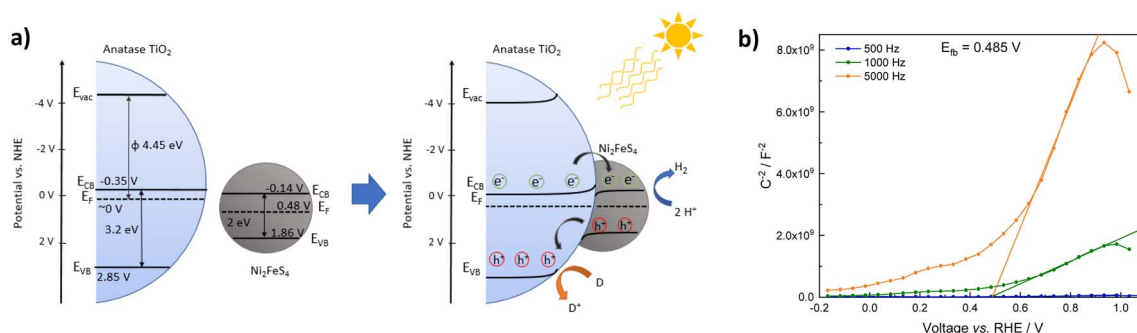
Fig. 7 Band positions of \text{TiO}_2 and \text{Ni}_2\text{FeS}_4 before and after contact (a) and Mott–Schottky plots for \text{Ni}_2\text{FeS}_4 in 0.5 \text{ M Na}_2\text{SO}_4 (values are already converted to pH 0) (b).
