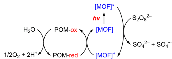
Scheme 4 Photocatalytic cycle of a \text{Co}_4\text{-POM@MOF} photosystem. 15
