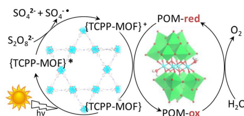
Scheme 5 Proposed mechanism for the light-driven water oxidation by \text{Porp-Co}_4@MOF-545 . Reprinted from ref. 84 with permission from American Chemical Society (Copyright 2018).
