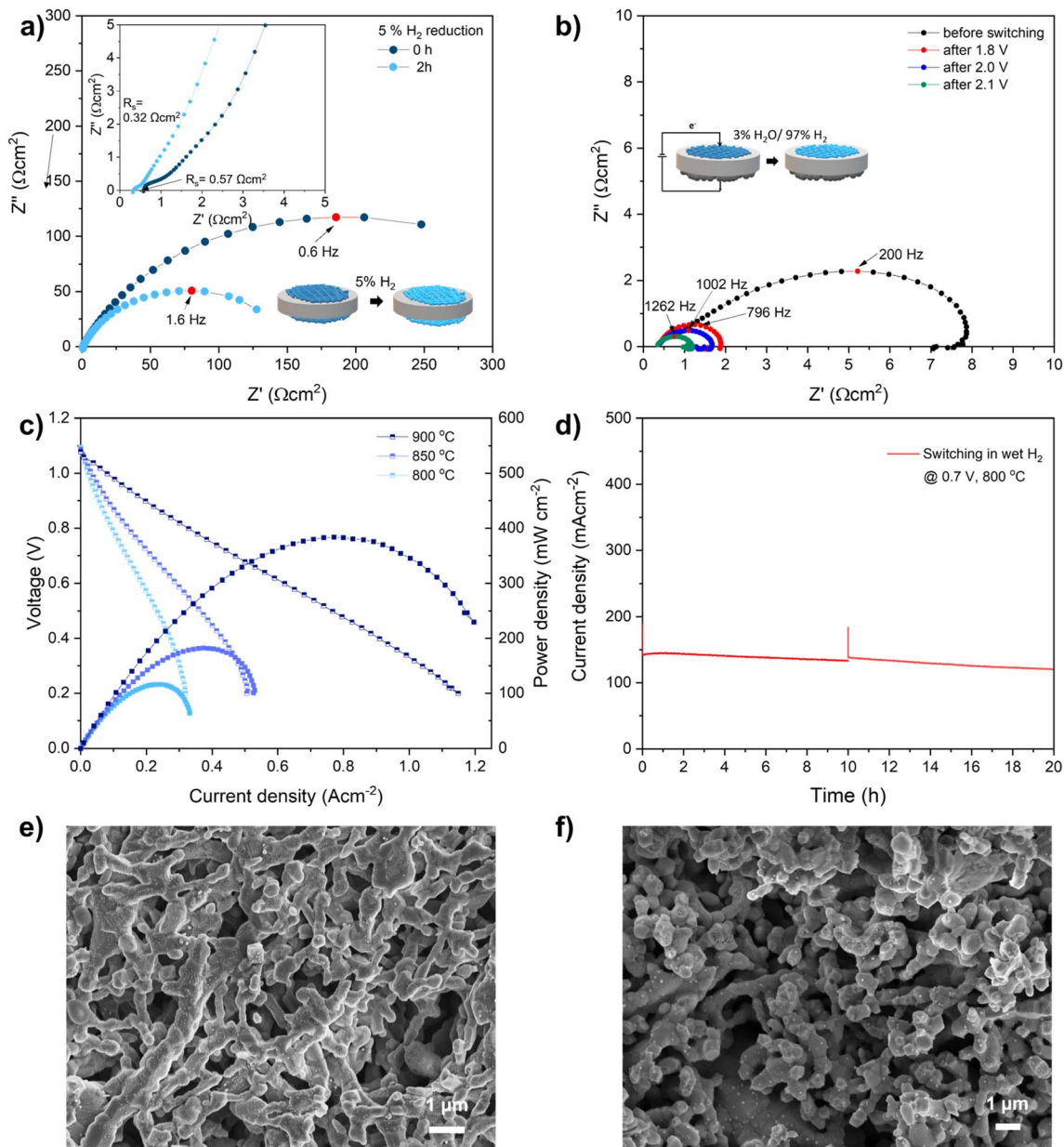
Fig. 5 Performance and short-term stability of fiber electrode-based fuel cells. (a) Impedance spectra of the symmetric cells reduced at 800 °C in 5% H 2 /N 2 for 0 and 2 h. (b) Impedance spectra after switching for 180 s at 900 °C at OCV in ~3% H 2 O/97% H 2 . (c) current–voltage–power curves of the cell at different temperatures after switching in wet H 2 . (d) Short term stability in wet H 2 for 20 h. SEM figure of (e) fiber electrode surface in symmetric cell after reduction, (f) fiber electrode in cell after stability test.
