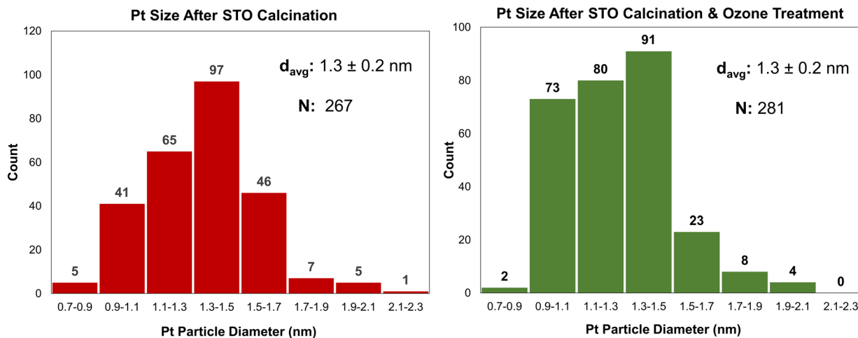
Fig. 4 Platinum particle size distributions for SOMC 1cPt/STO prepared with STO that had been calcined at 550 °C and steamed at 200 °C (red, average size of 1.3 ± 0.2 nm) and with an additional ozone treatment at 200 °C between the calcination and steaming steps (green, average size of 1.3 ± 0.2 nm). Metalation of MeCpPtMe 3 at 65 °C.
