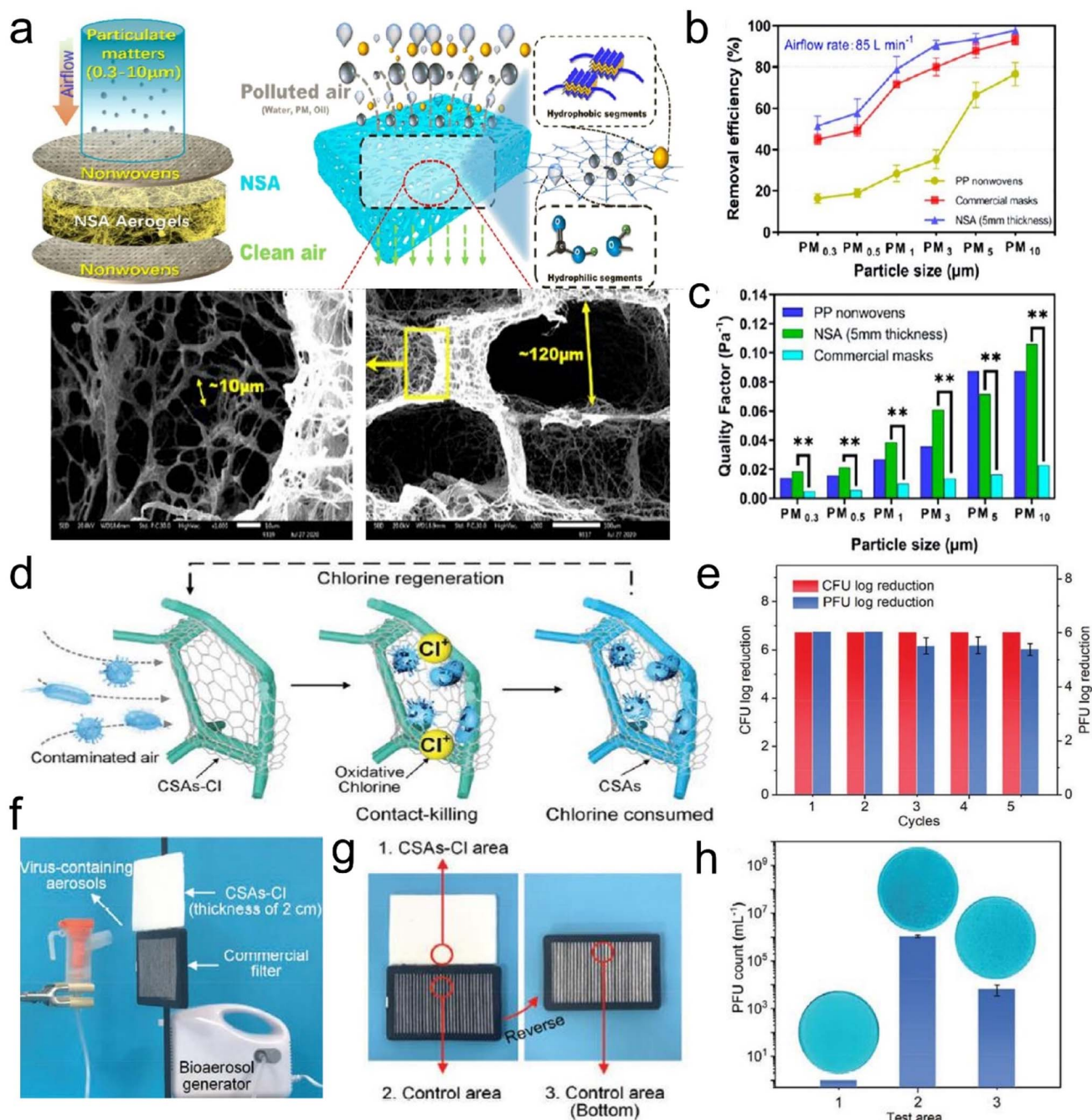
Fig. 13 3D fibrous aerogels used in air filtration. (a) Illustration of the contaminants captured by SNF aerogels. (b) Removal efficiency at 85 L \text{min}^{-1} for differently sized particles. (c) Quality factor of the three kinds of materials at 85 L \text{min}^{-1} for differently sized particles. Reproduced with permission. 88 Copyright 2021, American Chemical Society. (d) Illustration showing the air filtration procedure of the aerogels. (e) Renewable antibacterial and antiviral properties of CSAs-Cl. (f) Virus-containing aerosol generator and the antiviral test using an aerogel and 3 M filter. (g and h) The antiviral properties of the selected three areas of the filters. Reproduced with permission. 92 Copyright 2021, Wiley-VCH.
