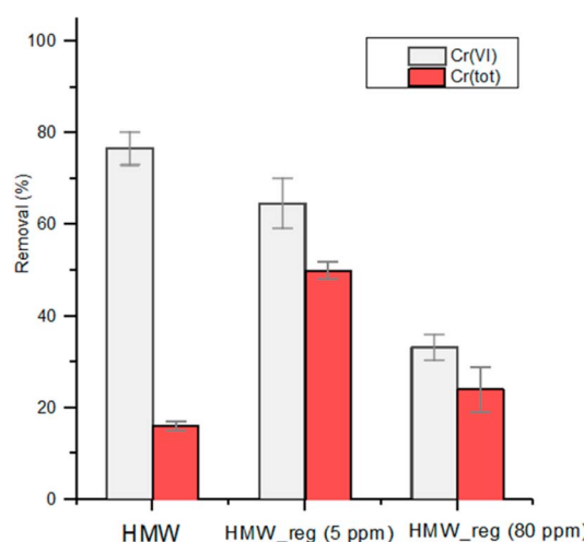
Fig. 7 Reduction of Cr(vi) by HMW and two regenerated lignins, HMW_reg_5 and HMW_reg_80. pH 2 obtained with 2 M HNO 3 ; 1 g L -1 of lignin; initial Cr(vi) concentration: 5 mg L -1 ; contact time: 2 h.
