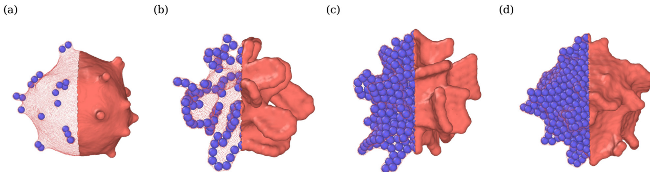
Fig. 3 Vesicle shapes in the near-equilibrium "cauliflower" regime at Pe = 15 and \varepsilon = 3.5k_B T for (a) \phi = 0.009 , (b) \phi = 0.04 (see Movie S4, ESI † ), (c) \phi = 0.12 , and (d) \phi = 0.18 . Different nearly-frozen structures of the ABPs are observed, including ring-like and sheet-like arrangements. The left half of the membrane is made transparent so that the arrangement of ABPs is visible.
