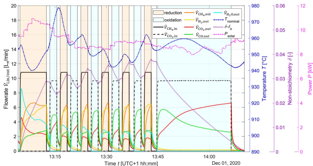
Fig. 6 Solar radiative power input, nominal temperature, inlet/outlet gas compositions, and \delta of CeO 2- \delta as a function of time during high- \delta redox reforming cycles. Flow rate data was smoothed using a local regression with weighted linear least squares and a 2nd degree polynomial. H 2 O flowrate data was determined via C : H ratio balance. To illustrate the high- \delta cycles, the \delta - \delta_0 plot is adjusted with the start point as \delta_0 and the subsequent values are linearly and uniformly shifted to ensure \delta_{\text{end}} - \delta_0 \approx 0 . In reality, \delta_{\text{end}} = 0.038 due to a gradual shift over the cycling.
