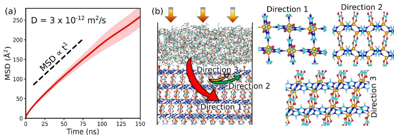
Fig. 5 CO 2 diffusion in the CALF-20/CMC composite by molecular dynamics simulations. (a) Mean-squared displacement of CO 2 in CALF-20/CMC for loading at 1 bar and 300 K. (b) Illustration of the diffusion mechanism with the CO 2 pathway along the three directions in CALF-20.
